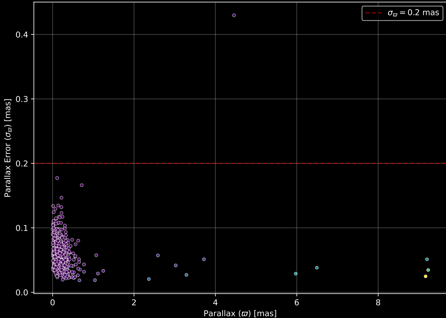
APOGEE DR17 Field: [340+06] Parallax Quality (n= 481)
