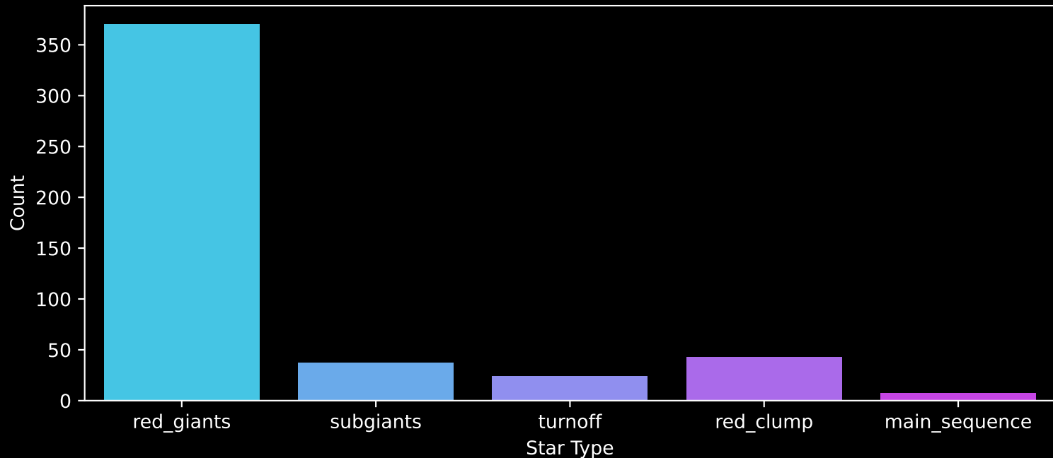
APOGEE DR17 Field: [340+06] Count plot of Star Type
