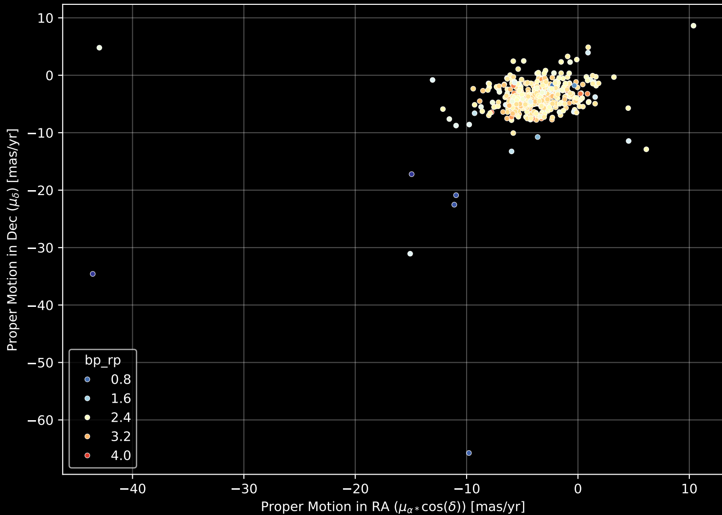
APOGEE DR17 Field: [340+06] Proper Motion Diagram (n= 481)
