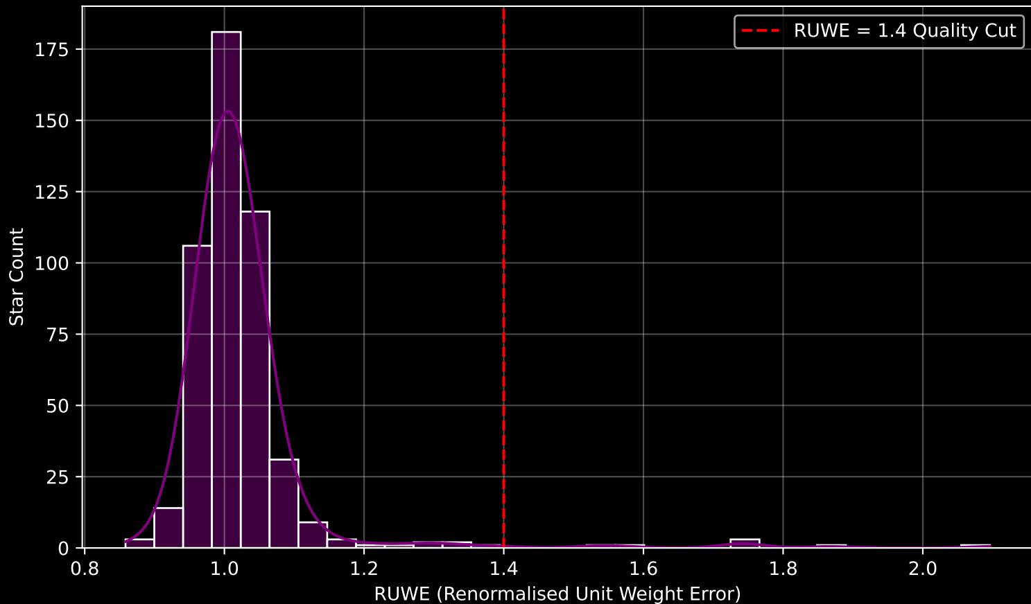
GAPOGEE DR17 Field [340+06] RUWE Distribution (n= 479)
