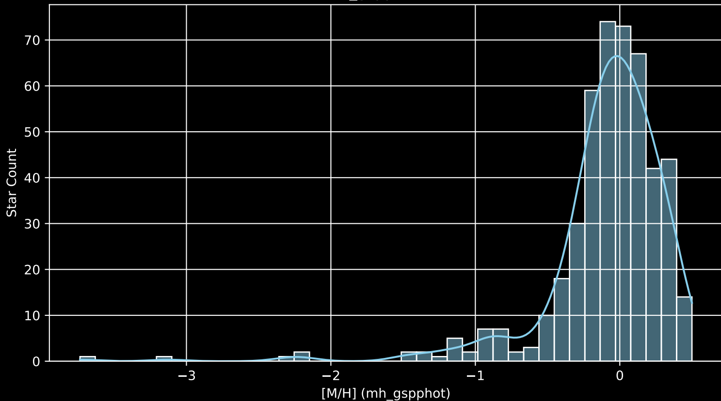
APOGEE DR17 Field: [340+06 [M/H] (mh_gspphot) (n= 467)
