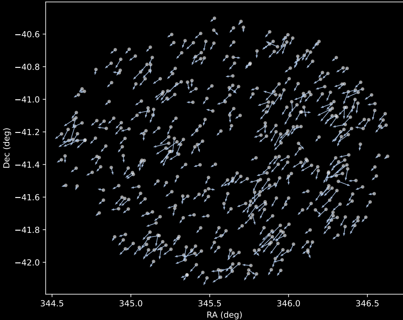
APOGEE DR17 Cluster 1 Proper Motion Vectors (n=454)
